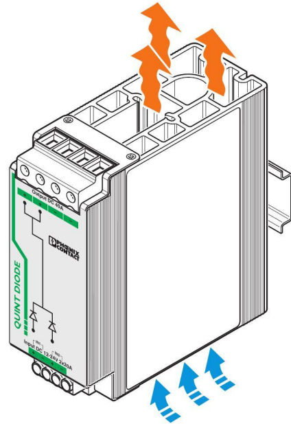
Figure 2 Convection
